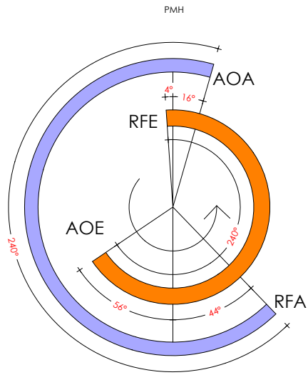
BMW R80GS/R100R
