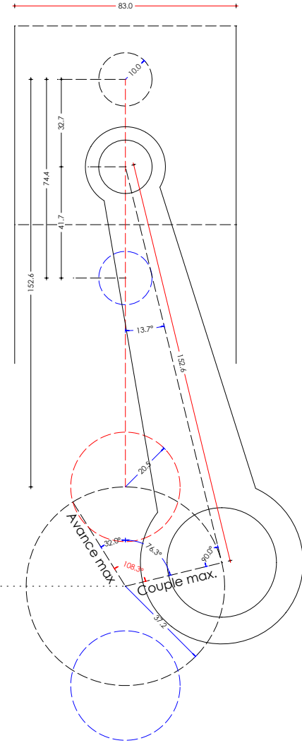
Suzuki VX/VS 800 GL Al x c: 83x74.4 Bielle longue 152.6 (>2x74.4) Rapport vol: 10:1
