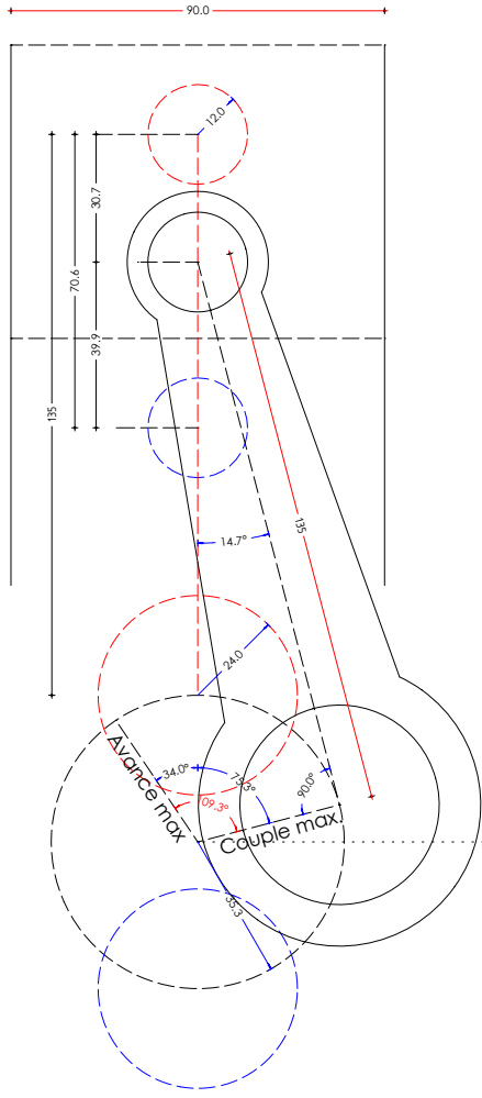
BMW R90S Al x c: 90x70.6 Bielle courte 135 (<2x70.6) Rapport vol: 9.5:1
